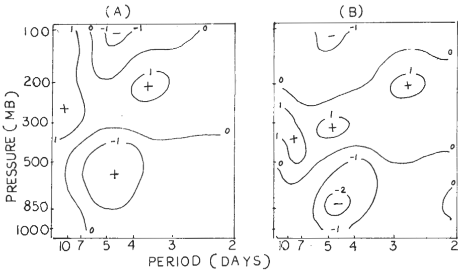
Fig 11. Vertical cross-section in cospectrum ( T' , v' ) for 1971 summer (unit: m\ sec^{-1}\ ^\circ K\ day ) (A)Tungkong (B)Makung
