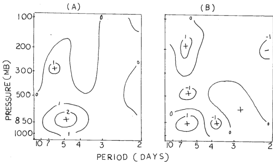
Fig 12. Vertical cross-section in cospectrum ( T' , v' ) for 1972 summer (unit: m\ sec^{-1}\ ^\circ K\ day ) (A)Taoyuan (B)Tungkong
