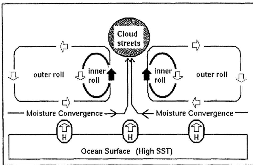
Sketch of the relationship between convective rolls and cloud streets
