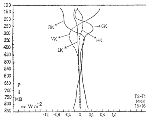
Fig. 15(c). Same as Fig. 14, except for the area of 15 \times 16 grids.
