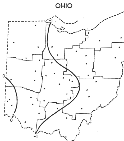
Fig. 8. Thirty-year temperature change, annual. (°F) (1931-1960 mean minus 1861-1890 mean)
