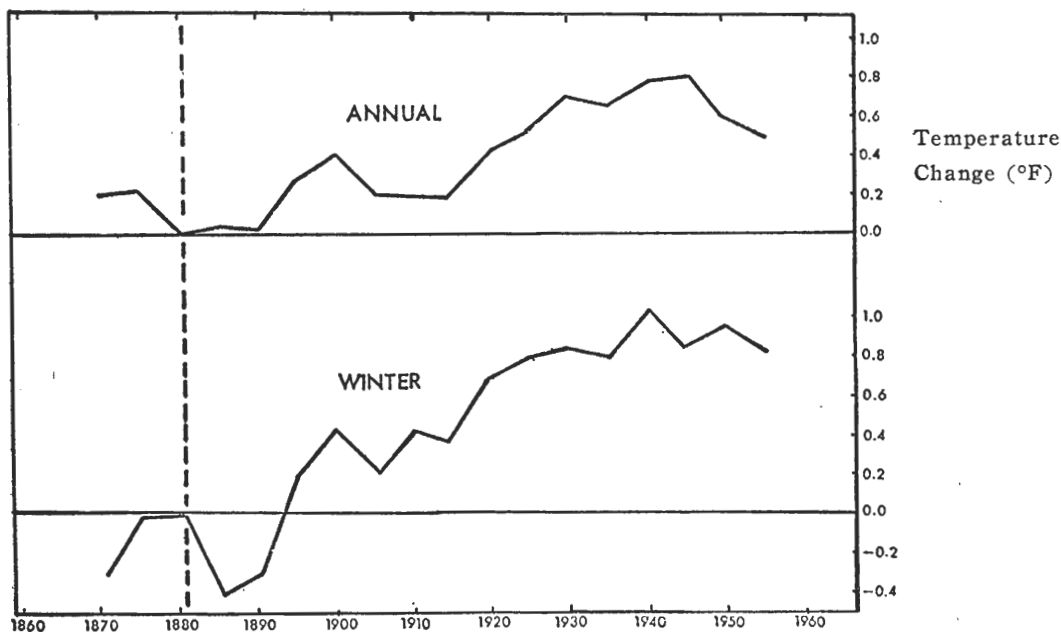
Fig. 1. Trends of mean temperature in 0°-60°N, shown for successive pentads relative to the 1880-1884 pentad (after Mitchell).
