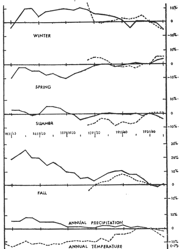
Fig. 11. Thirty-year moving averages of seasonal and annual weighted average precipitation departures from 1931-1960 normals (in percent of normal amount).
